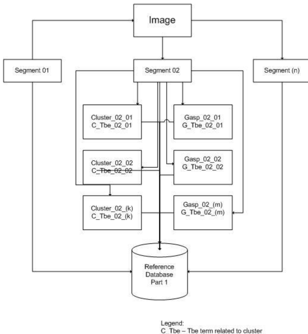
Fig.3 Semantic network concerning to information capability of the actual image which consists of clusters and segments (SNIC).
